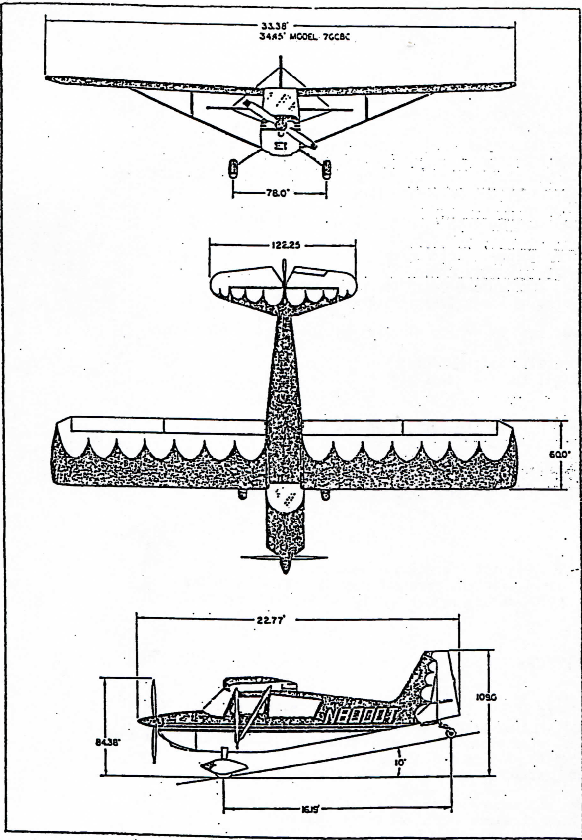
FIGURE 6-2 CITABRIA THREE-VIEW
